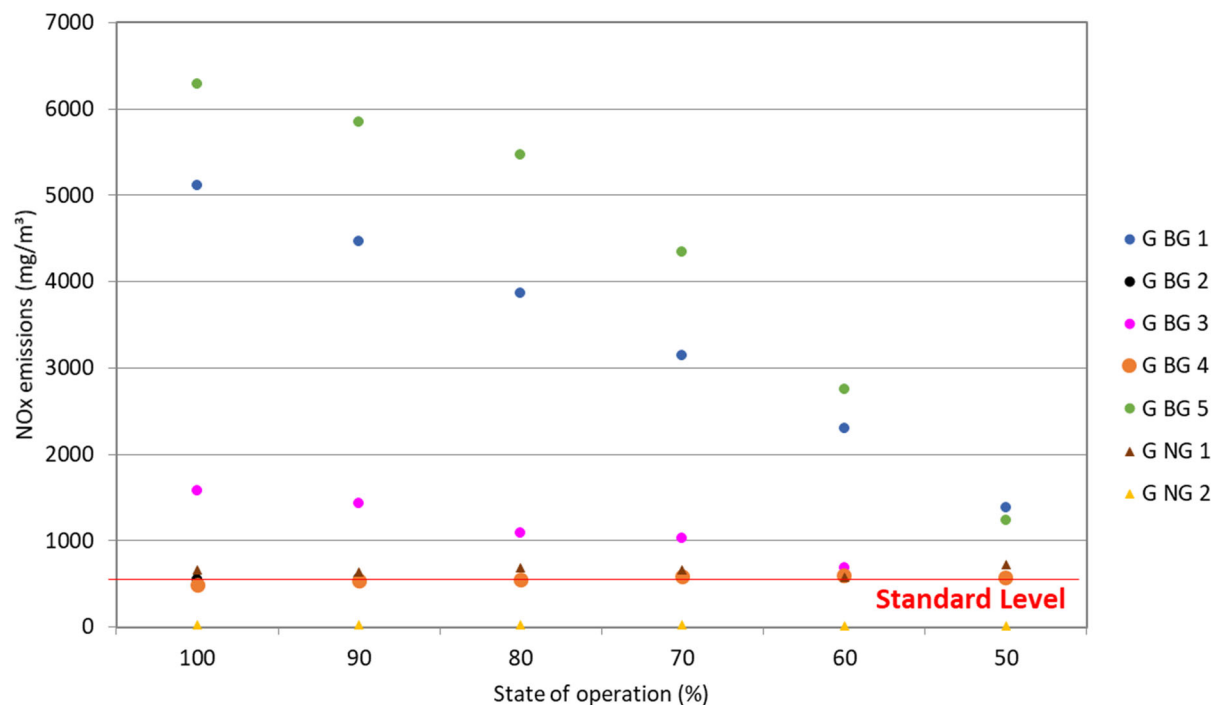
Fig.10 The NO x emissions during step responses
