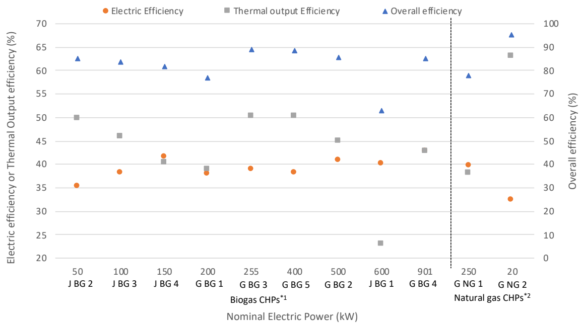
Fig.4 Electric, Thermal output and overall Efficiency of the CHP systems
