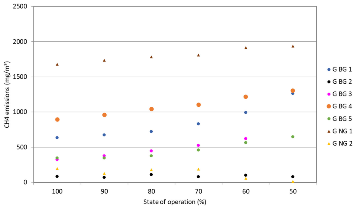
Fig.11 The \text{CH}_4 emissions during step responses
